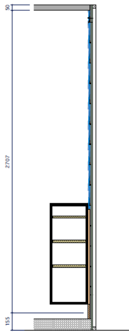
[断面図-c] S=1/20
