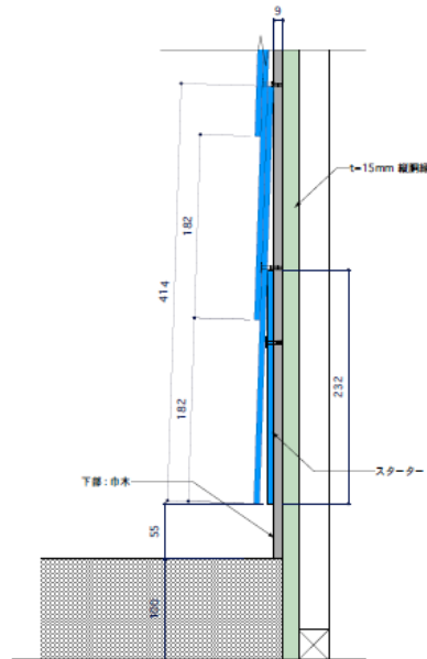
[断面図-c_下部] S=1/5
