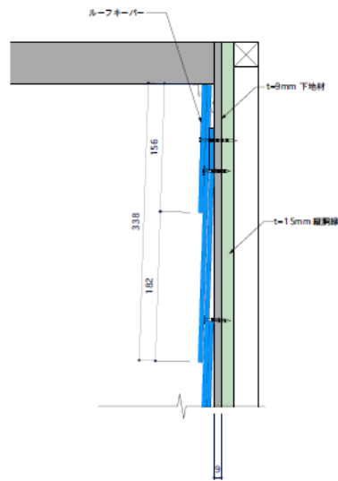
[断面図-c_上部] S=1/5
